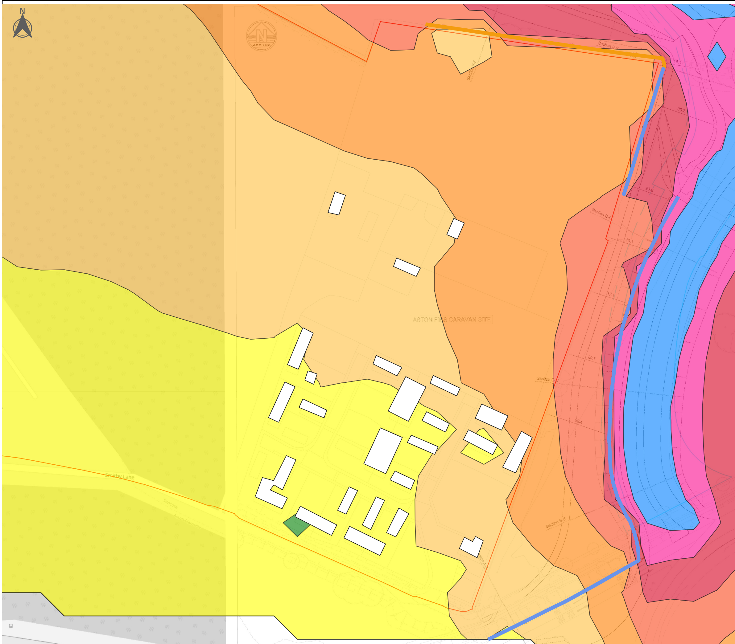
Figure 10.15A - Indicative Noise Contour - Operational Noise dB LAeq,1hr and A47 Link Road dB LAeq,16h with Mitigation
